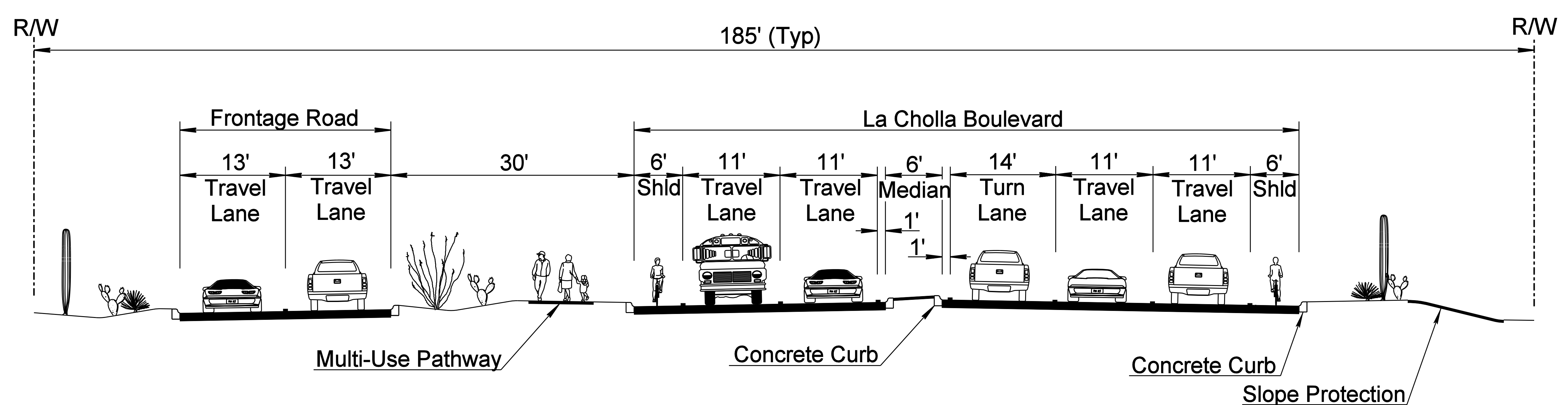
La Cholla Boulevard Roadway Typical Section (Near The Bluffs Subdivision)
