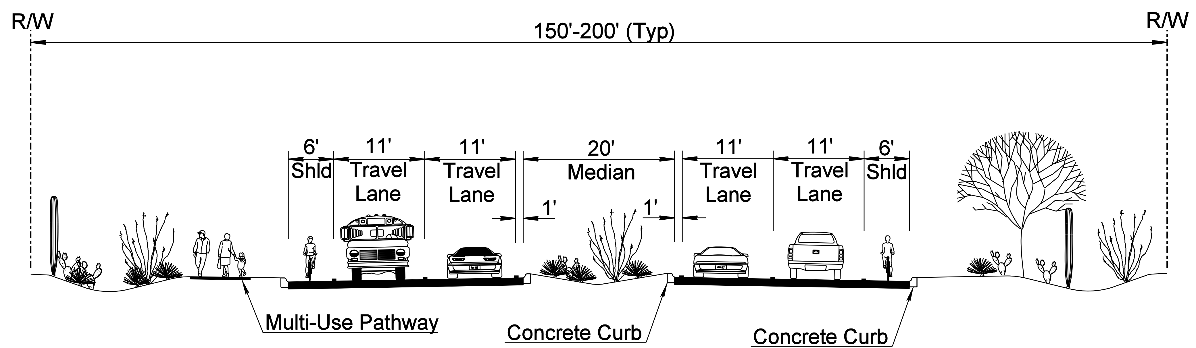
La Cholla Boulevard Roadway Typical Section
