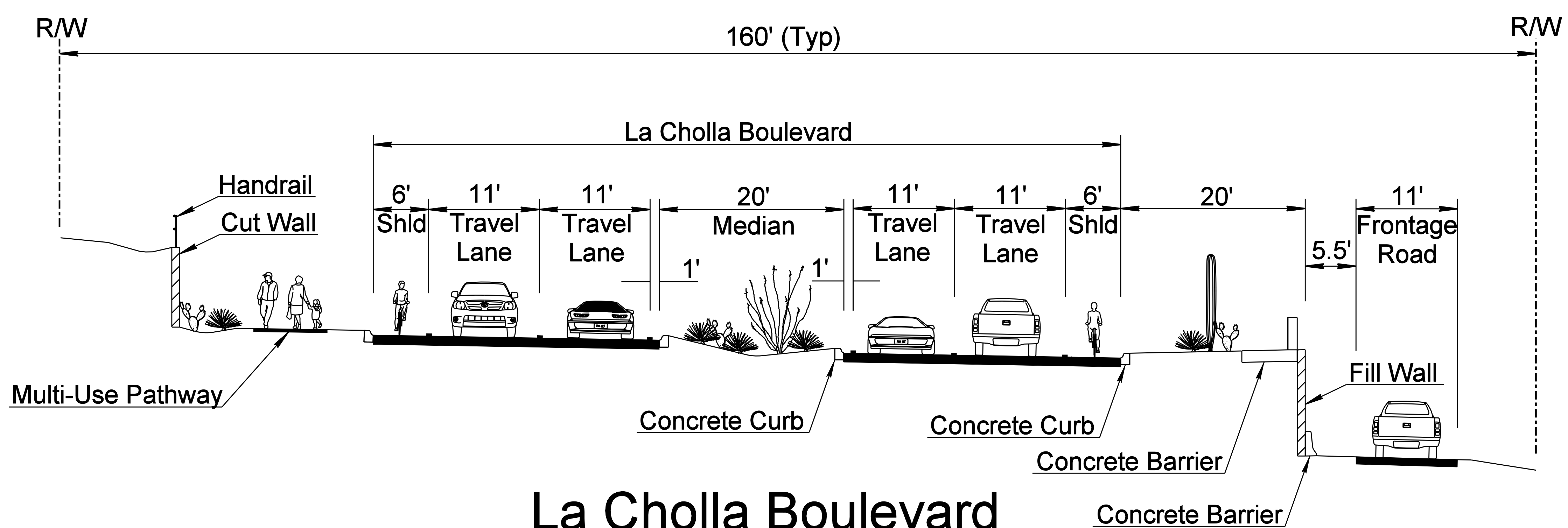
La Cholla Boulevard Roadway Typical Section (Near The Bluffs Subdivision)
