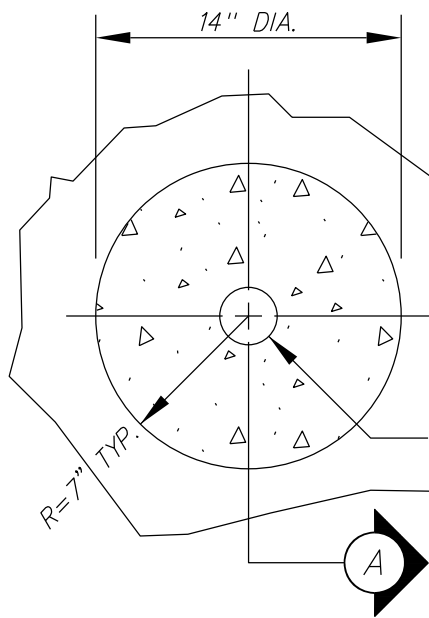
PLAN VIEW PREFERRED OPTION
