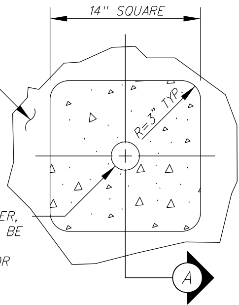
PLAN VIEW ALTERNATE OPTION
